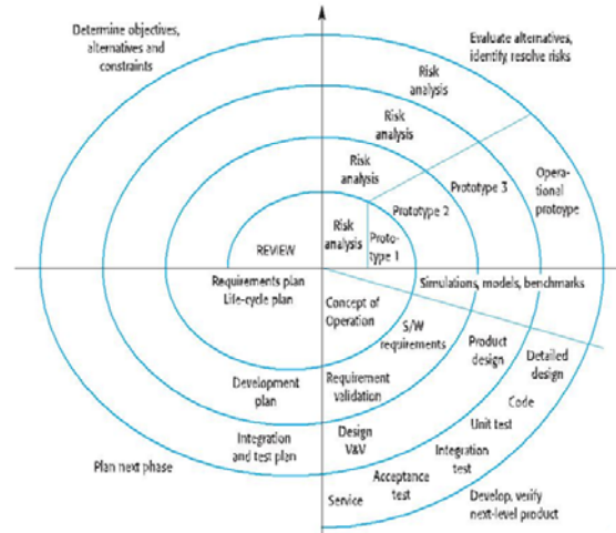
Fig. 7 Spiral Model of the Software Process[1].
