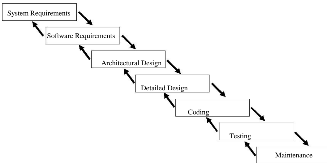
Fig. 2 Waterfall Model [4].
