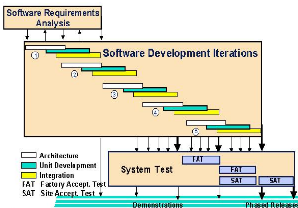
Fig. 4 Iterative Development.
