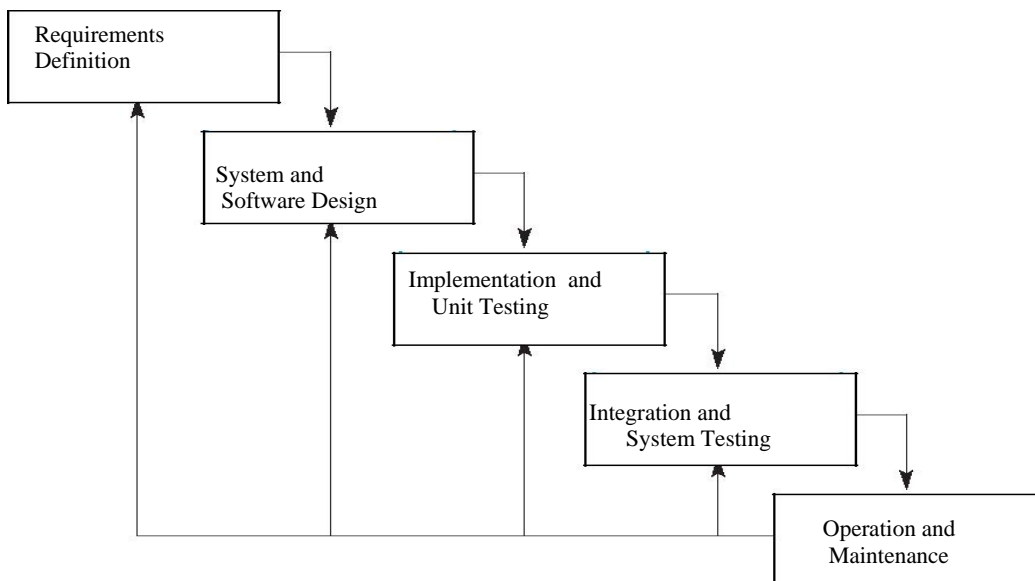
Fig. 3 Waterfall model [2].
